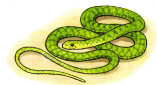
serpens (m)
